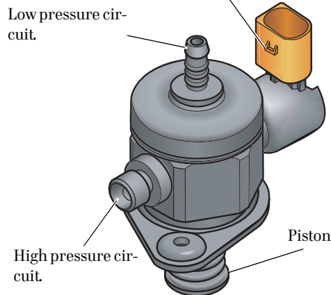
Fuel pressure regulator solenoid valve N276
