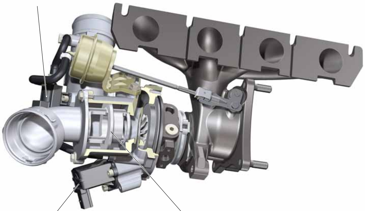
Turbocharger air recirculation solenoid valve N249
