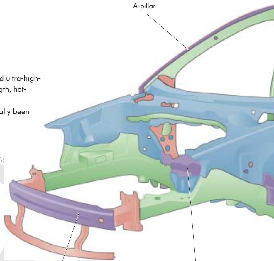
Cross members in the footwell area
