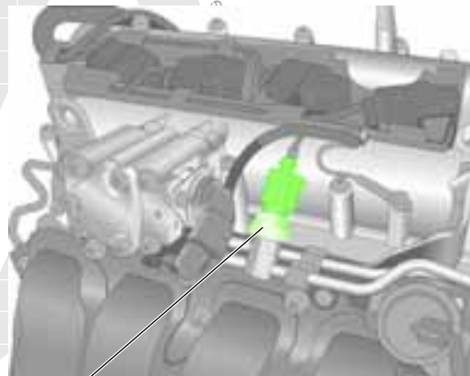
Fuel pressure sender, vacuum pressure G410
