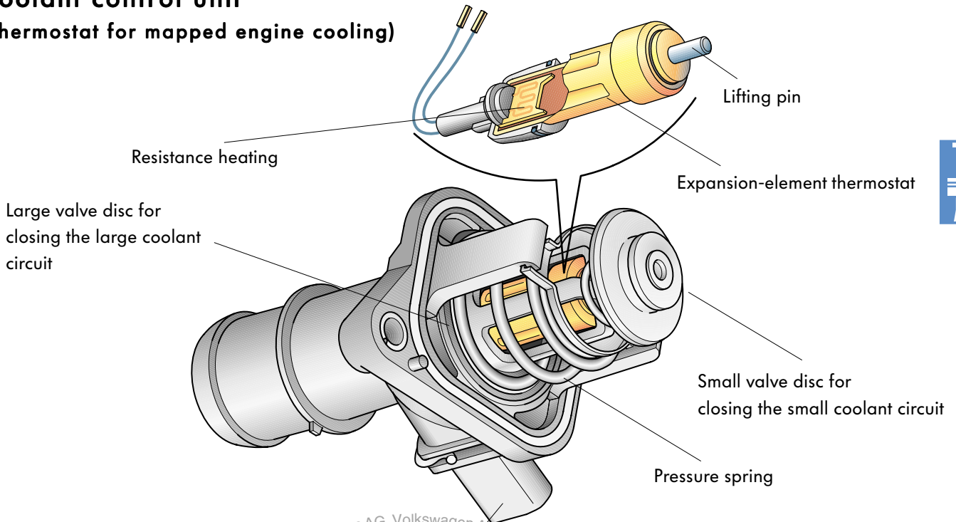
Connection between expansion-element thermostat and heating
