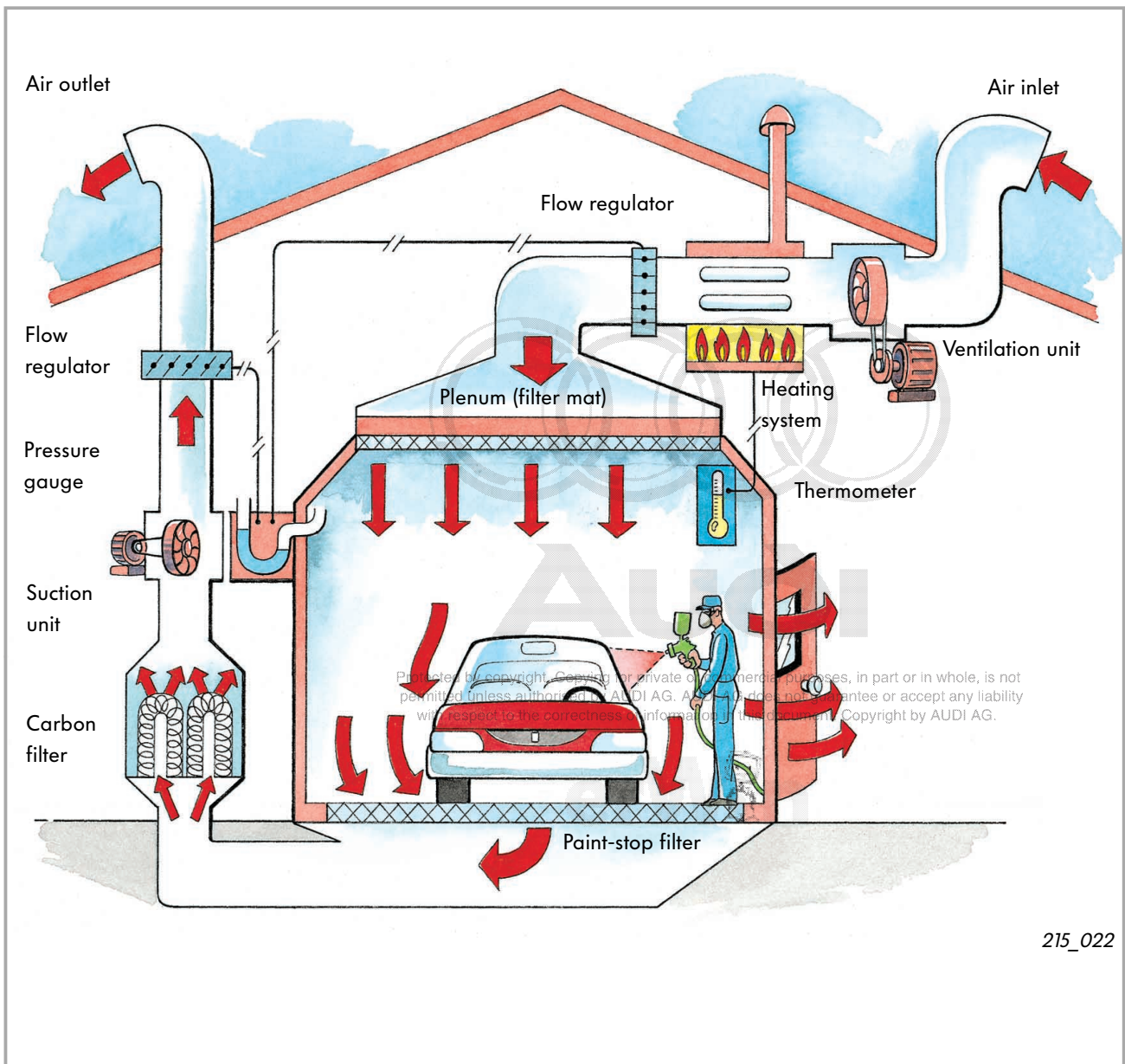
Spray chamber
