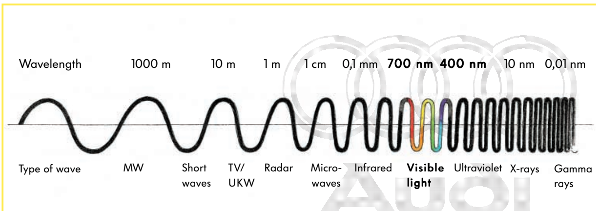
Electromagnetic rays
