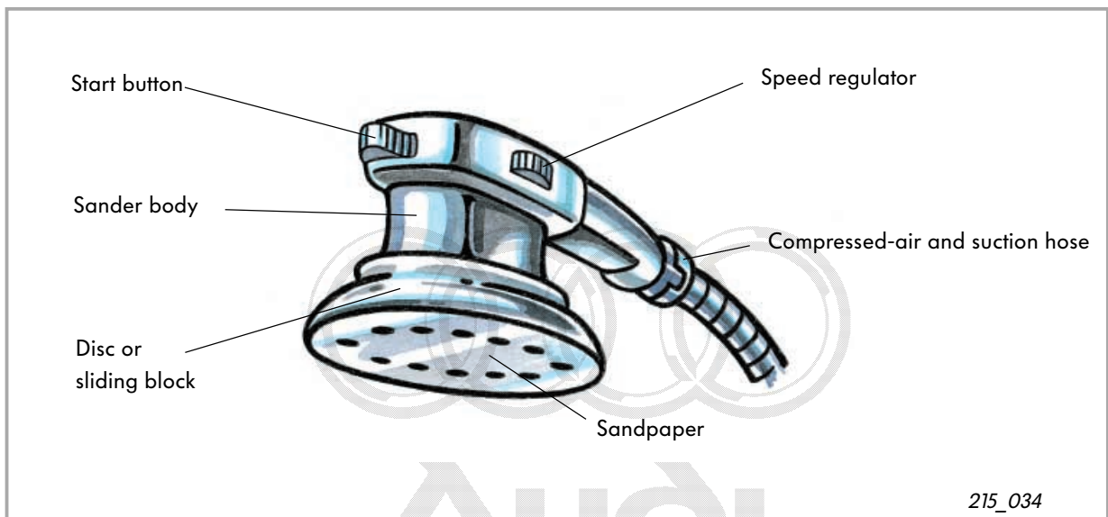
Pneumatic sander
