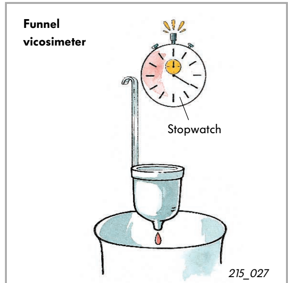
Viscosity-measuring beaker
