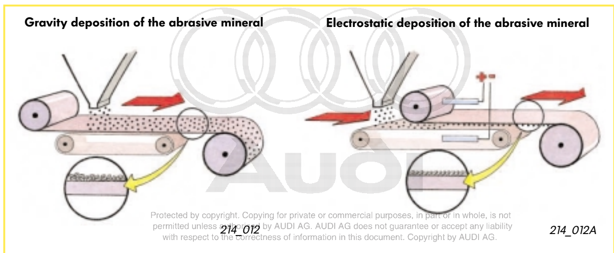
Gravity application and electrostatic application
