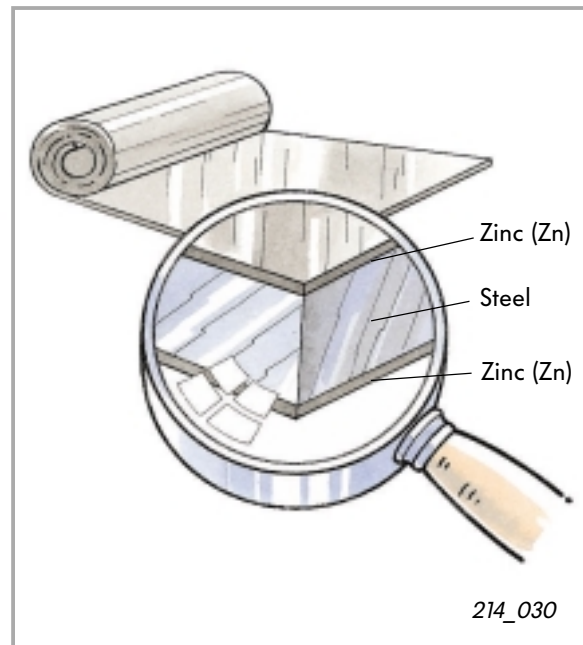
Double-sided galvanised steel panel
