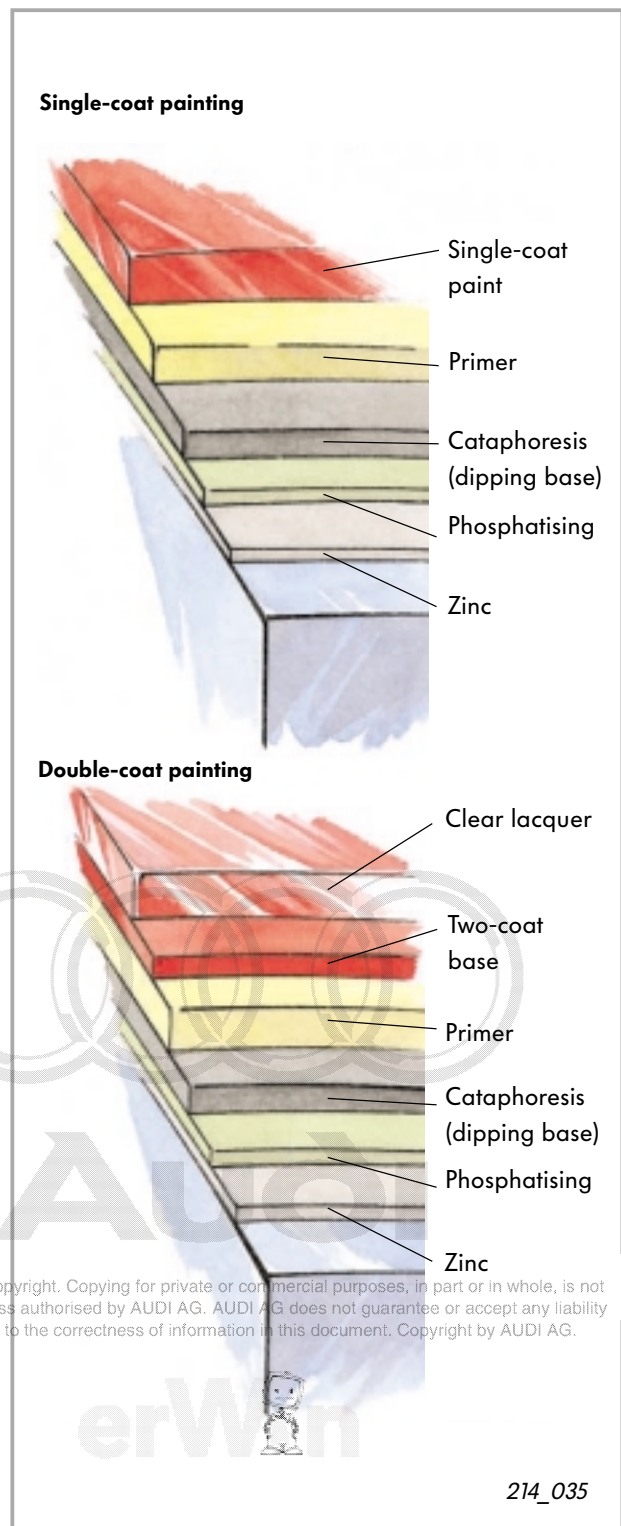
One-coat and two-coat paints
