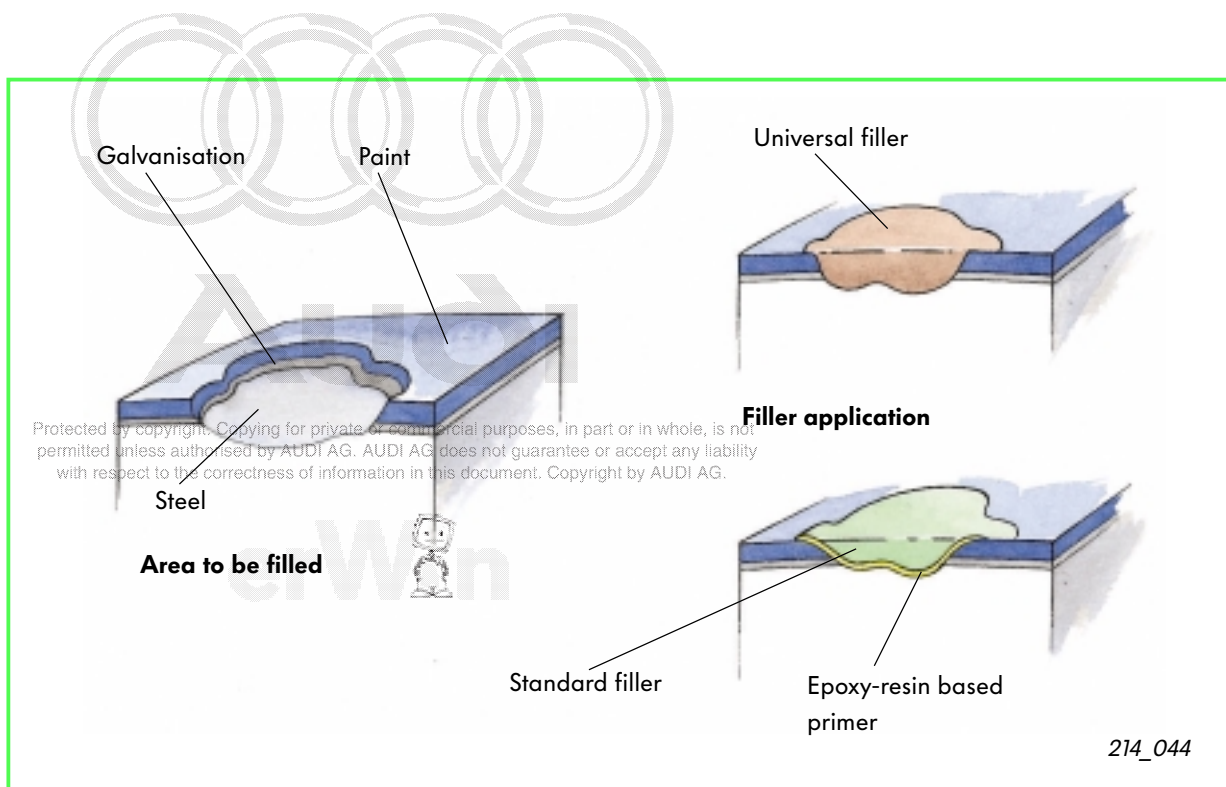
Application of filler on a galvanised panel
