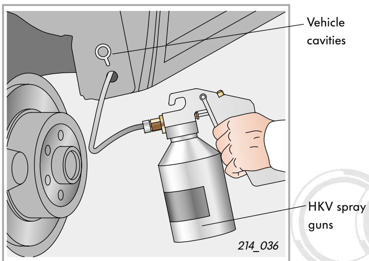
Cavity-conservation gun
